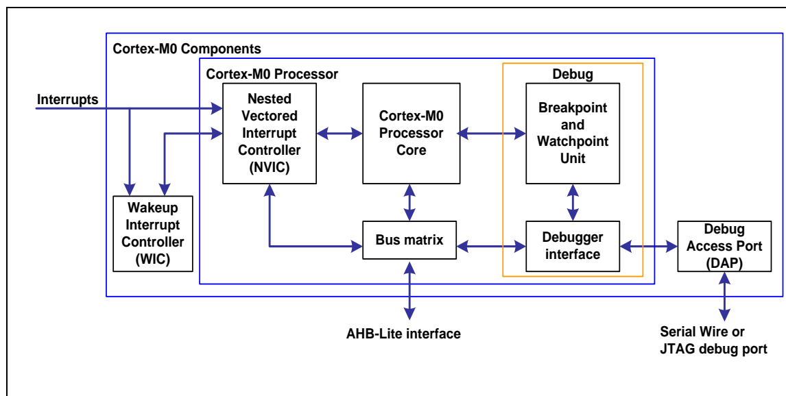
Figure 6-1 Functional Block Diagram
