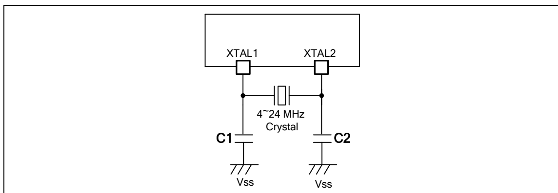
Figure 8-1 M05xxDN Typical Crystal Application Circuit
