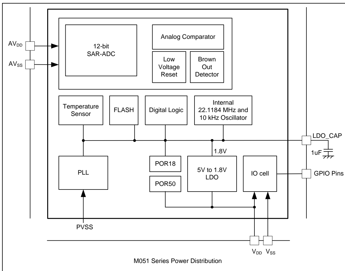
Figure 6-2 NuMicro® M051 DN/DE Series Power Architecture Diagram
